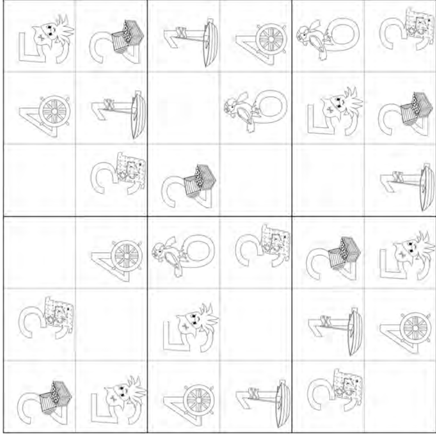
Puzzle 4 6x6 Very Easy
