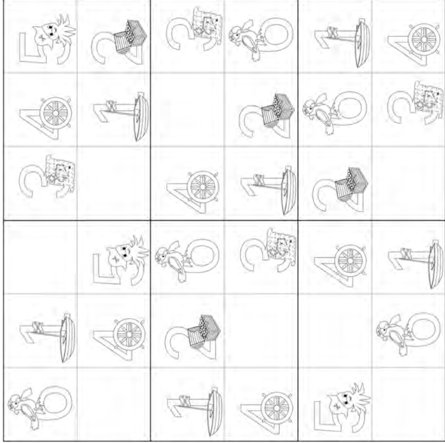
Puzzle 11 6x6 Very Easy
