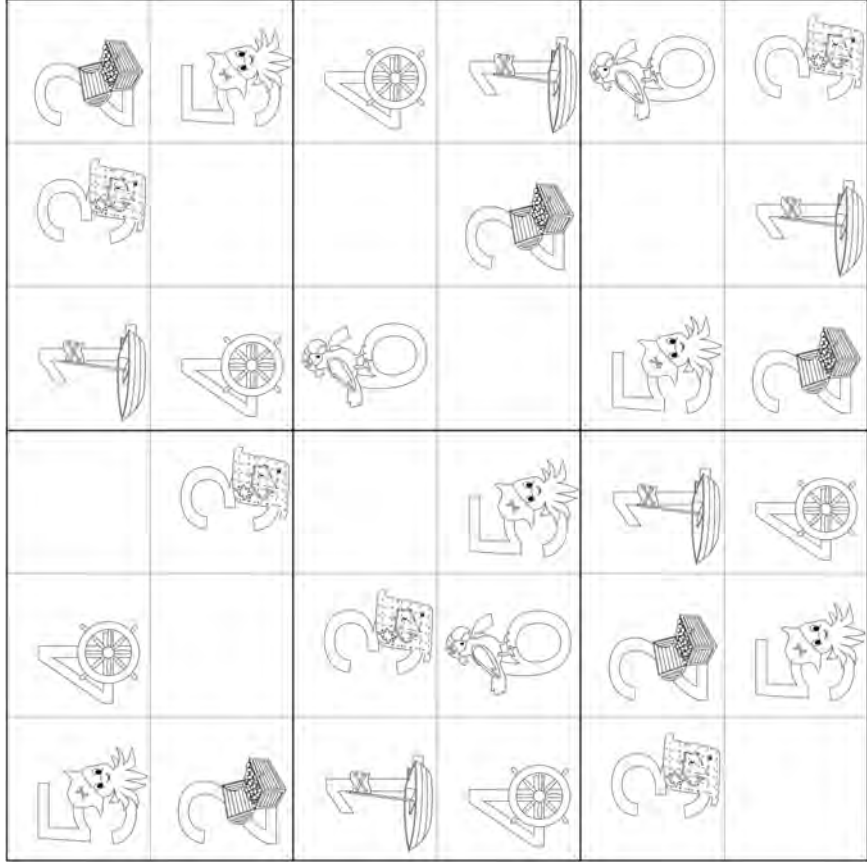
Puzzle 12 6x6 Very Easy
