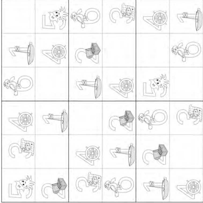
Puzzle 3 6x6 Very Easy
